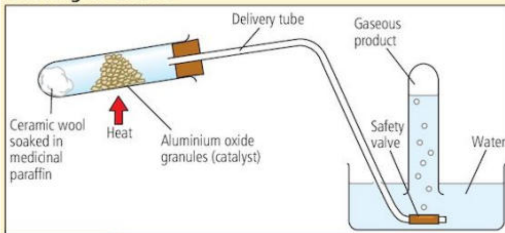
Figure 18.2.2 Aluminium oxide catalyses the cracking of alkanes
